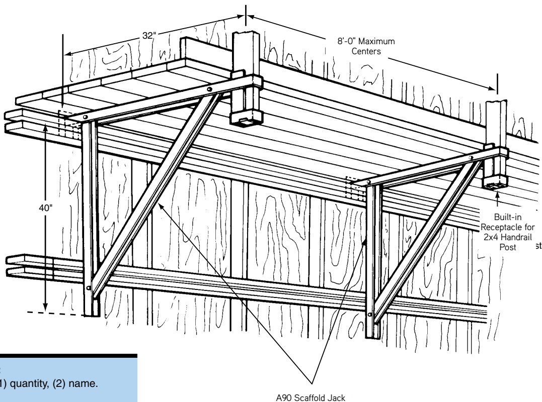
A90 Scaffold Jack
