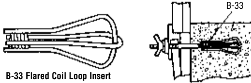
B-33 Flared Coil Loop Insert
